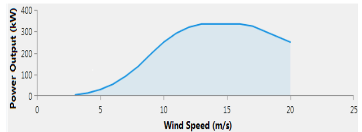
Figure 6: The wind turbine power curve
