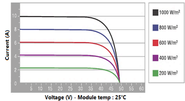
Figure 7: I-V characteristic of the photovoltaic generator for different radiations
