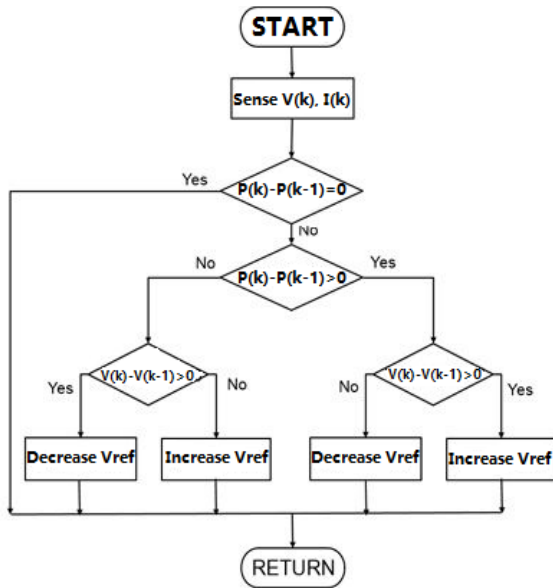
Figure 9: The perturbation and observation (P&amp;O) algorithm
