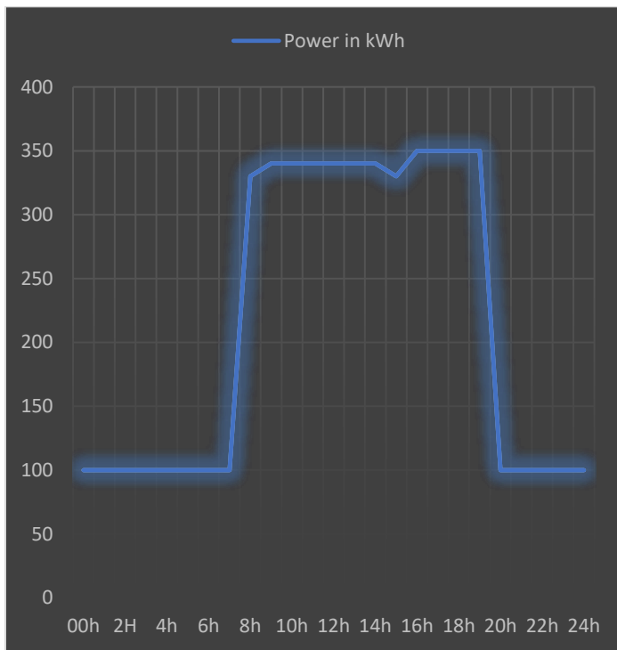
Figure 5: Electricity consumption profile
