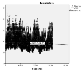
Figure 11: Relationship between temperature and time
